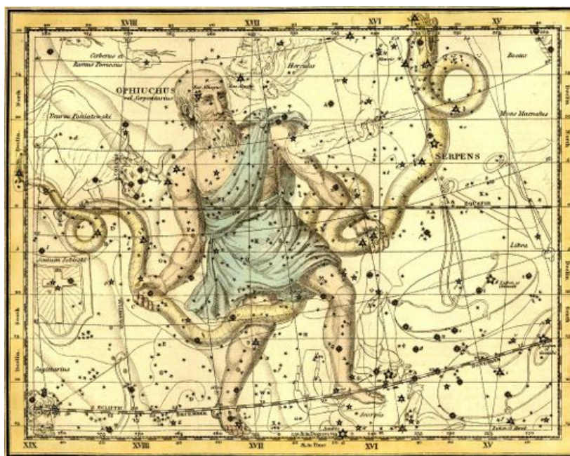
Ophiuchus
