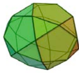
Icosidodecahedron 20 triangular faces and 12 pentagonal faces
